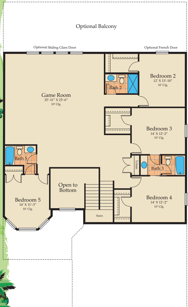
Second Floor
